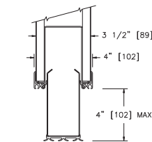
Optional Bottom Seal: 4" clearance
